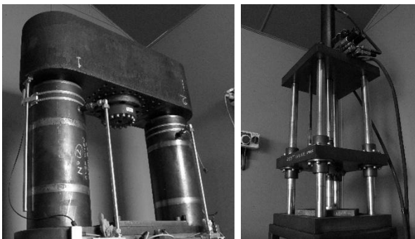
Remotely operated precision 180t and 10t presses.
